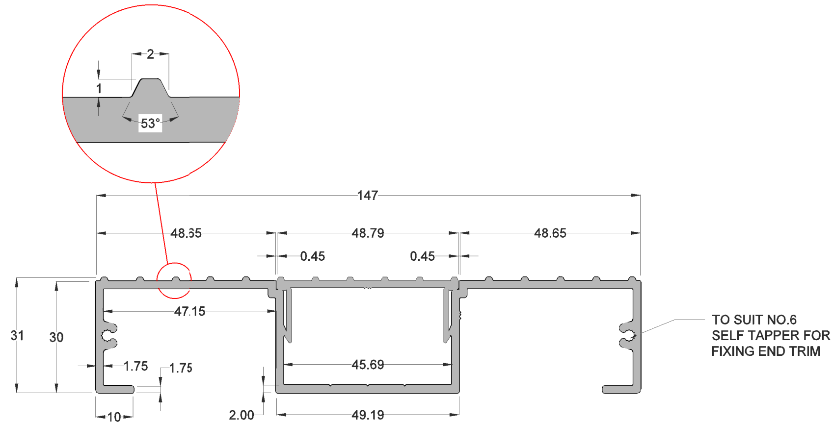
DECKBOARD DETAILS
