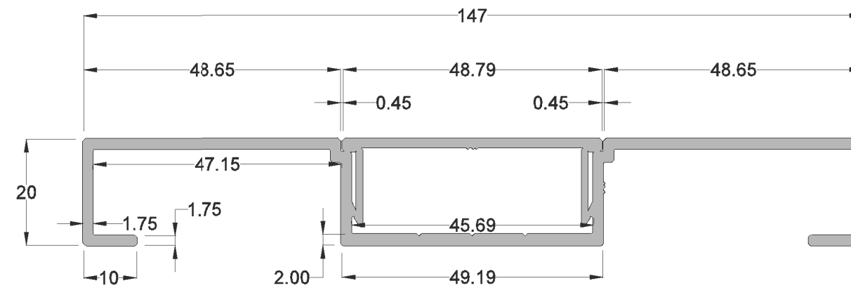
DECKBOARD DETAILS
