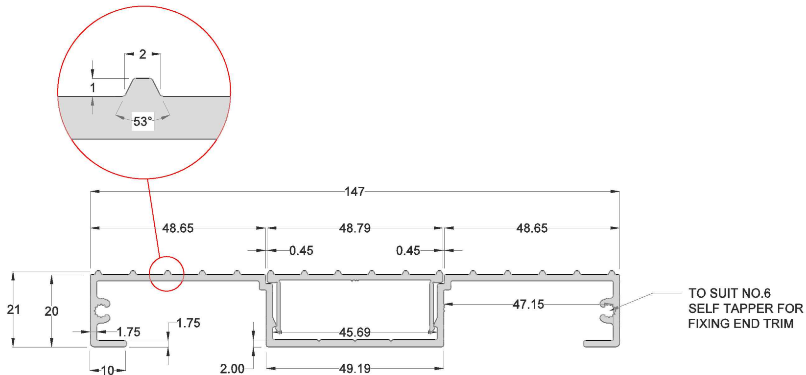
DECKBOARD DETAILS
