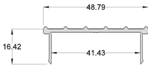
CHANNEL COVER DETAILS
